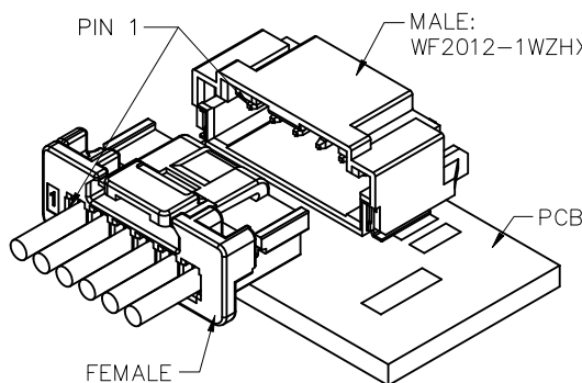
EXPLODED VIEW
