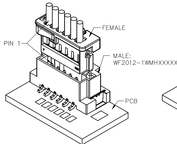
EXPLODED VIEW
