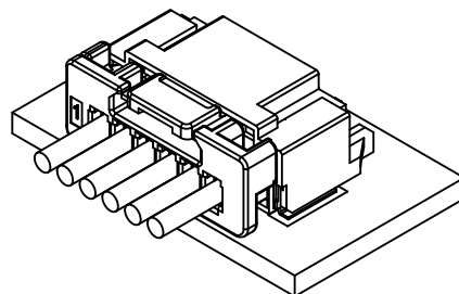
MATING VIEW
