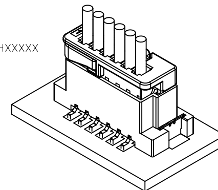
MATING VIEW
